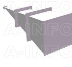
LB-137-25-C-NFSPO Standard Gain Horn Antenna 5.85-8.2GHz 25dB Gain N Type Female
